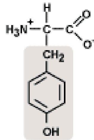
Tyrosine (Tyr)
